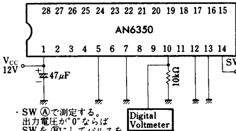
Test Circuit 10 ( V_{10} )
