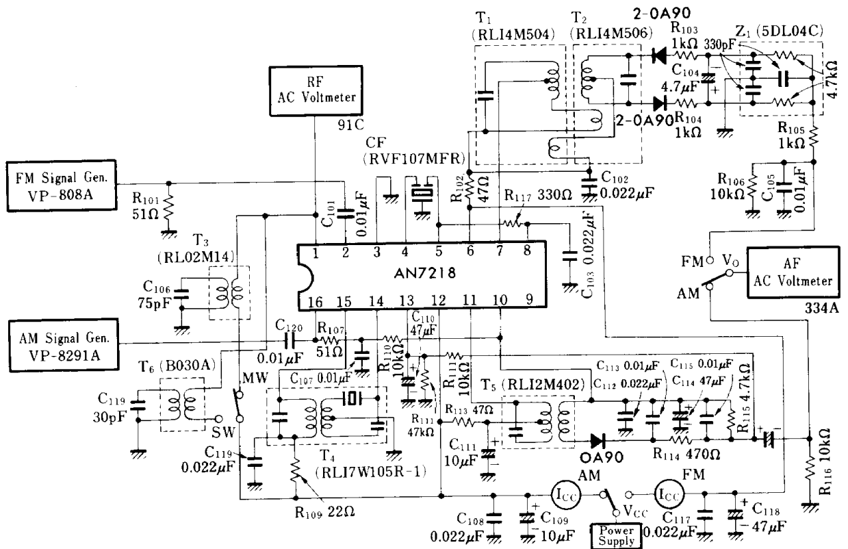
Test Circuit 1
