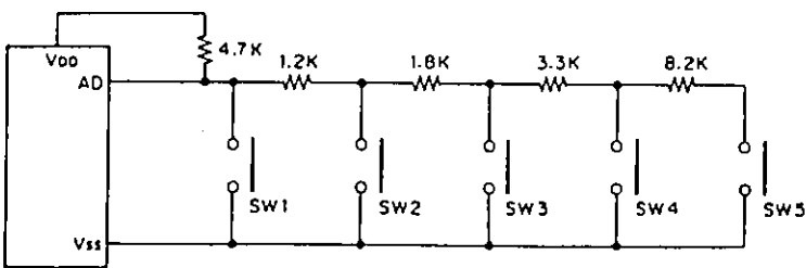
Fig.14 Recommended example of key input circuit by A/D converter
