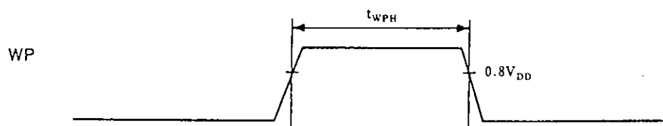
Fig.10 Wake-up input timing
