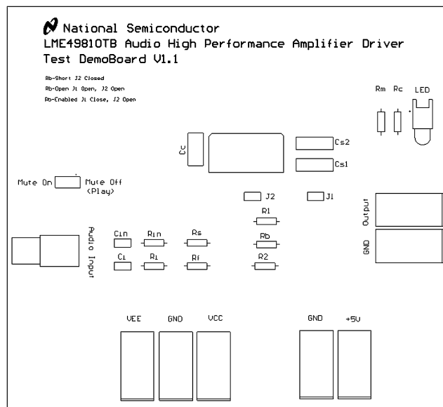
Figure 6. Silkscreen Layer
