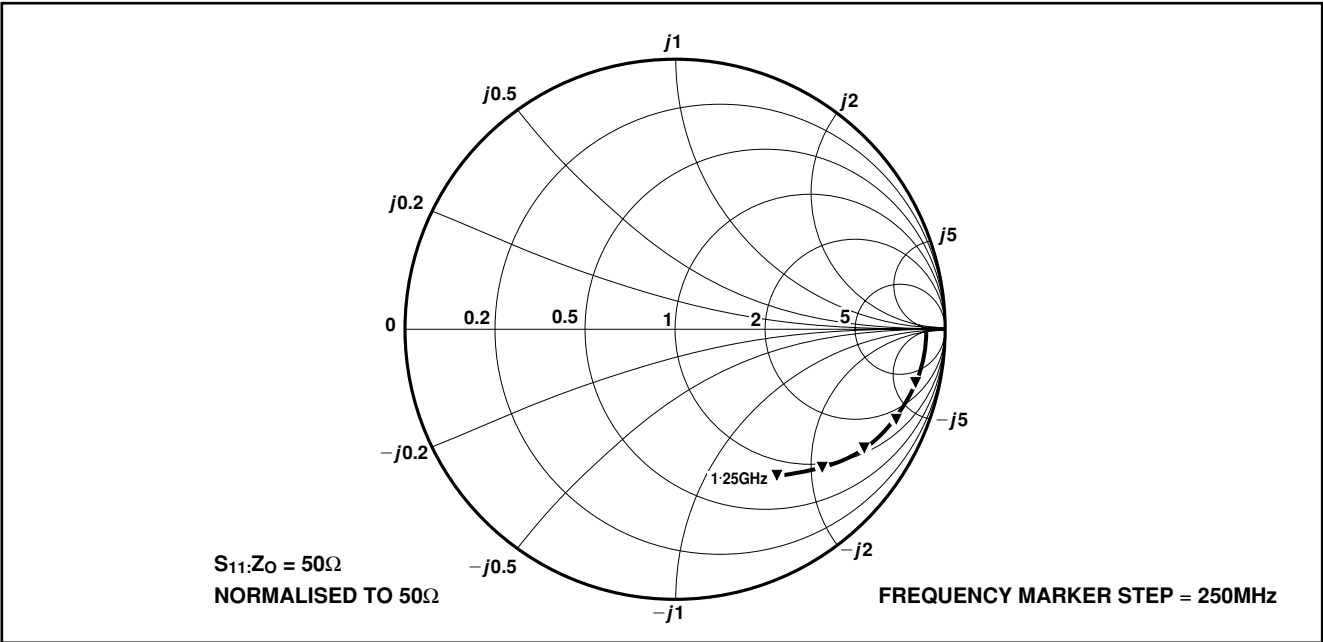
Fig. 8 Typical input impedance, SP5510S
