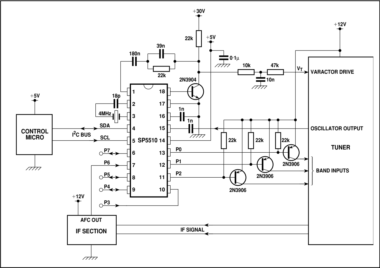
Fig. 4 Typical application
