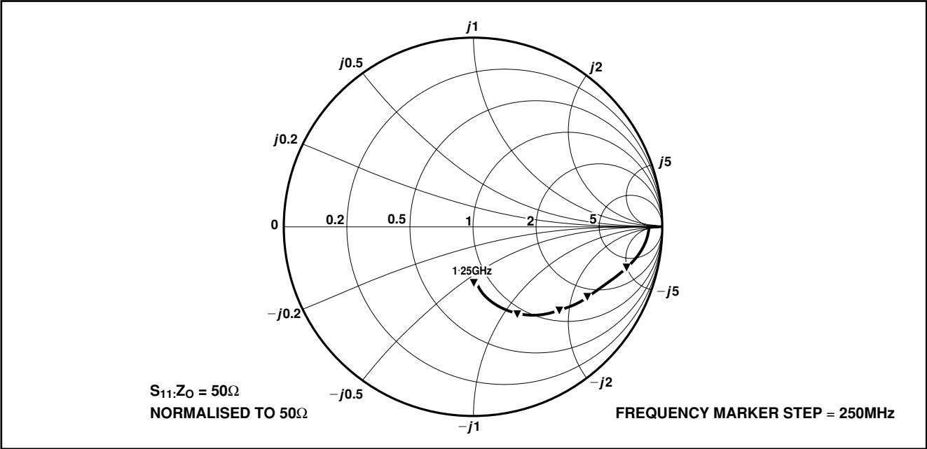
Fig. 7 Typical input impedance, SP5510
