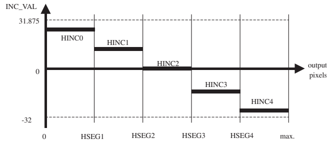
Fig. 2–44: Visualization of horizontal panorama segments
