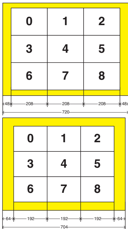
Fig. 2-50: Examples of 9 x 1/9 multi picture
