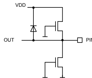
Fig. 4-19: Analog Output Pins: CVBSO1...CVBSO3
