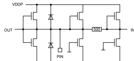
Fig. 4–15: Digital Input/Output Pins: 656IOX, 656CLK, 656HIN/CLKF20, 656VIN/BLANK
