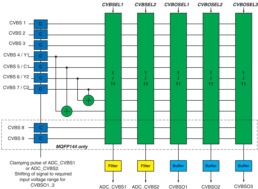
Fig. 2-3: Input selection
