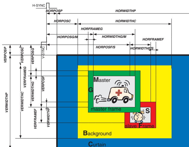
Fig. 2–61: Example of pixel mixer output
