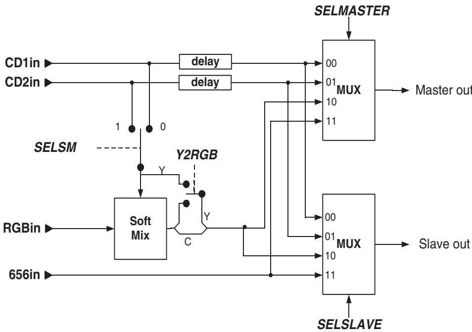
Fig. 2–27: Channelmux
