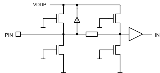
Fig. 4–13: Digital Input Pins: V, TMS, ADR/TDI, RESET, TCLK
