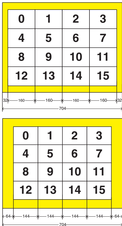
Fig. 2-51: Examples of 16 x 1/16 multi picture
